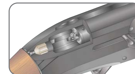
AN ELASTOMER BUFFER AT THE RECEIVER REAR prevents battering with heavy loads. Beretta's self-compensating gas valve lets you shoot the full range of today's ammunition.
