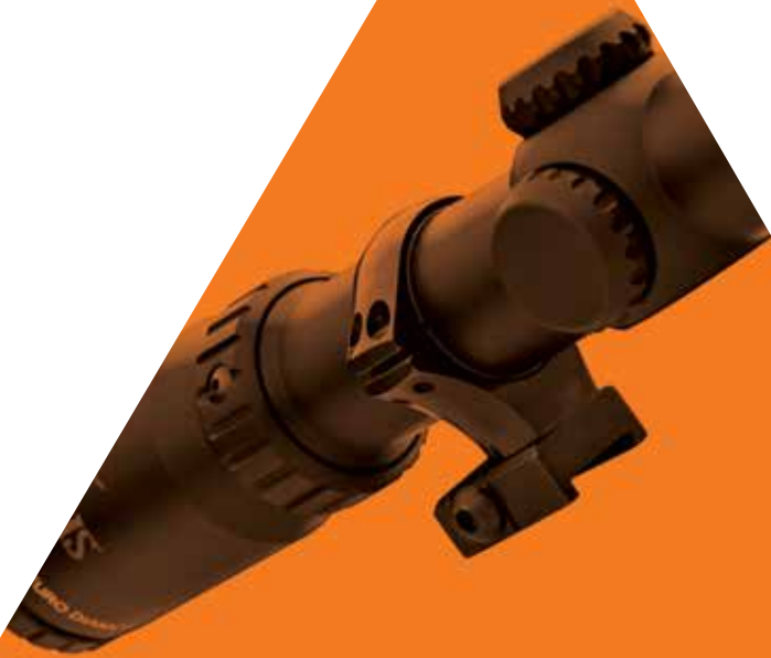
The front base of the Optilock has a limiter pin for the receiver's surface in front. This ensures correct remounting of the scope and Optilock unit, without requiring new sight adjustments if the unit is removed and repositioned.
